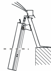
ESSMANN skylight dome with console for a 300 mm stroke ESSMANN servomotor opener.
